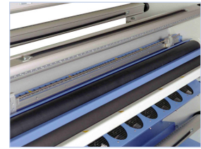
Cantilevered Supply Shaft (62 Pro S)
